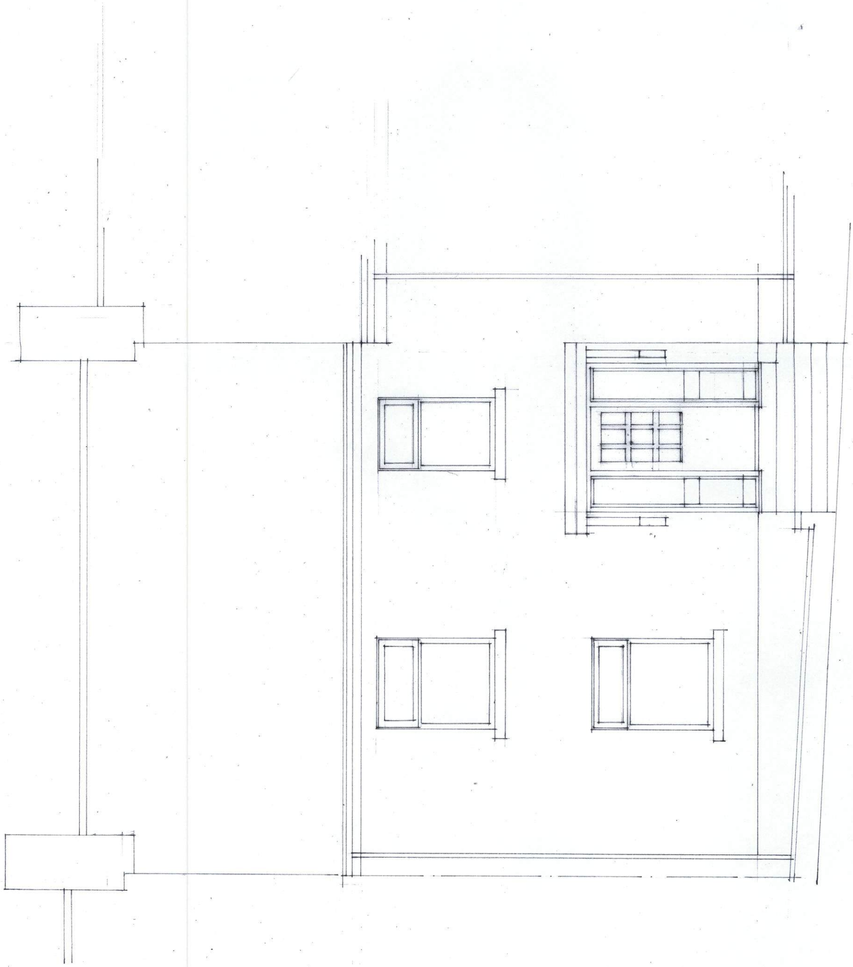
NORTH ELEVATION
